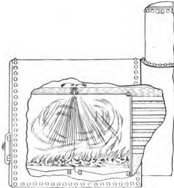
FIG. 125. —Part section through a large horizontal stationary boiler, showing the fire box and flue space. A fusible plug set at the highest fire line is melting, thus allowing the water and steam to escape into the fire box, extinguishing the fire. Fusible plugs will not melt so long as the water level is at the right height.
